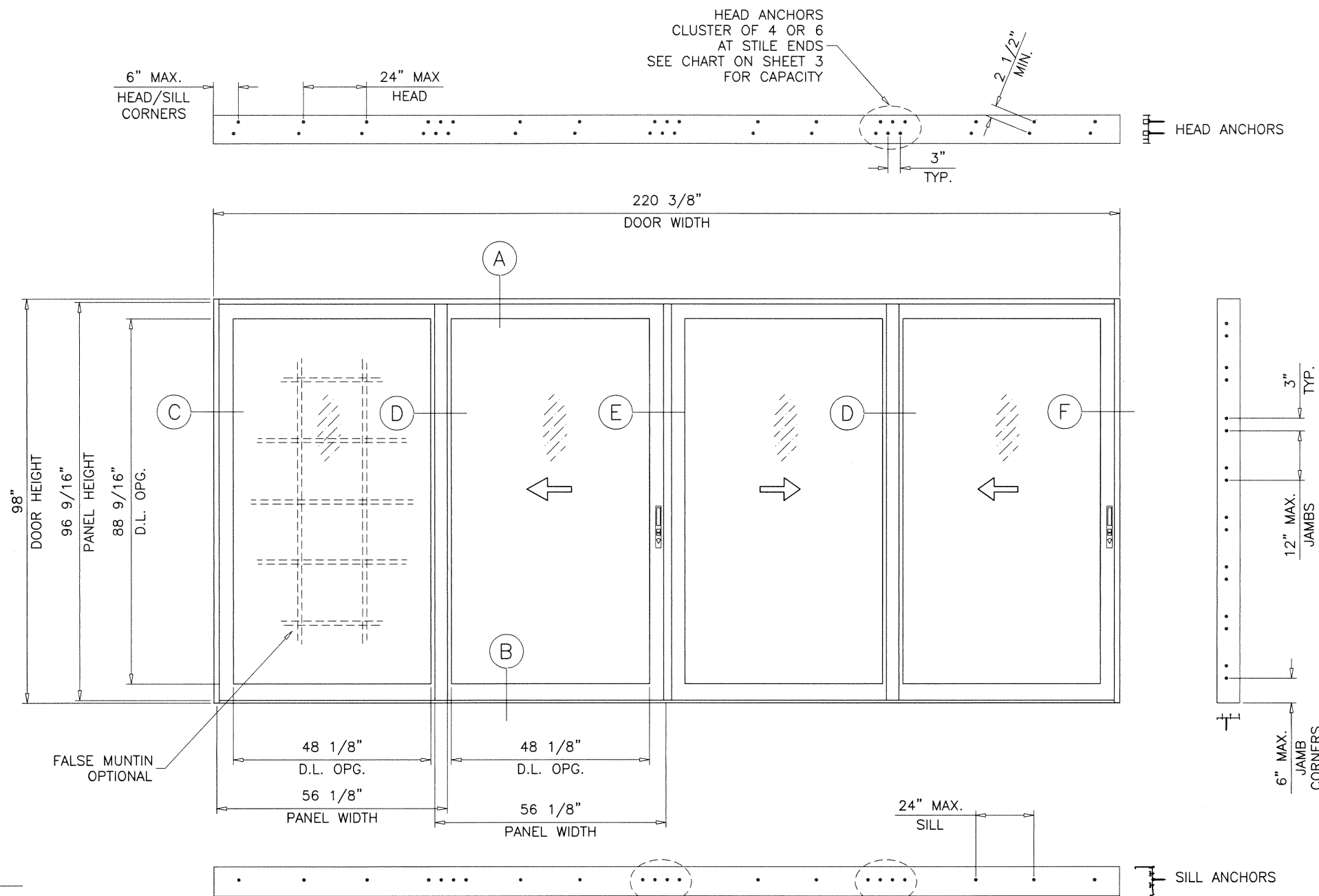
TYPICAL ELEVATION 2 TRACK FRAMES
