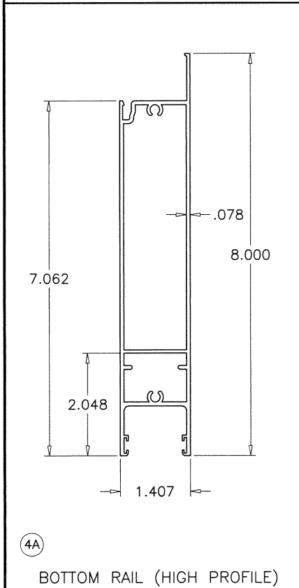
4 PANEL TOP & BOTTOM RAIL
