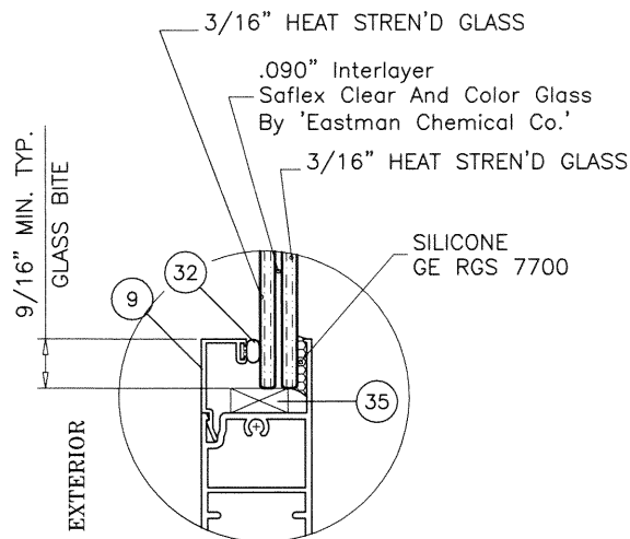
GLASS TYPE 'G1'
