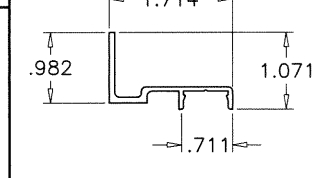
10 FIX. PANEL CLIP
