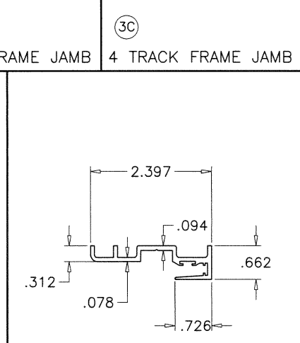
POCKET DOOR HOOK (TRIMMED)
