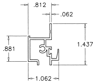
FIXED RAIL
