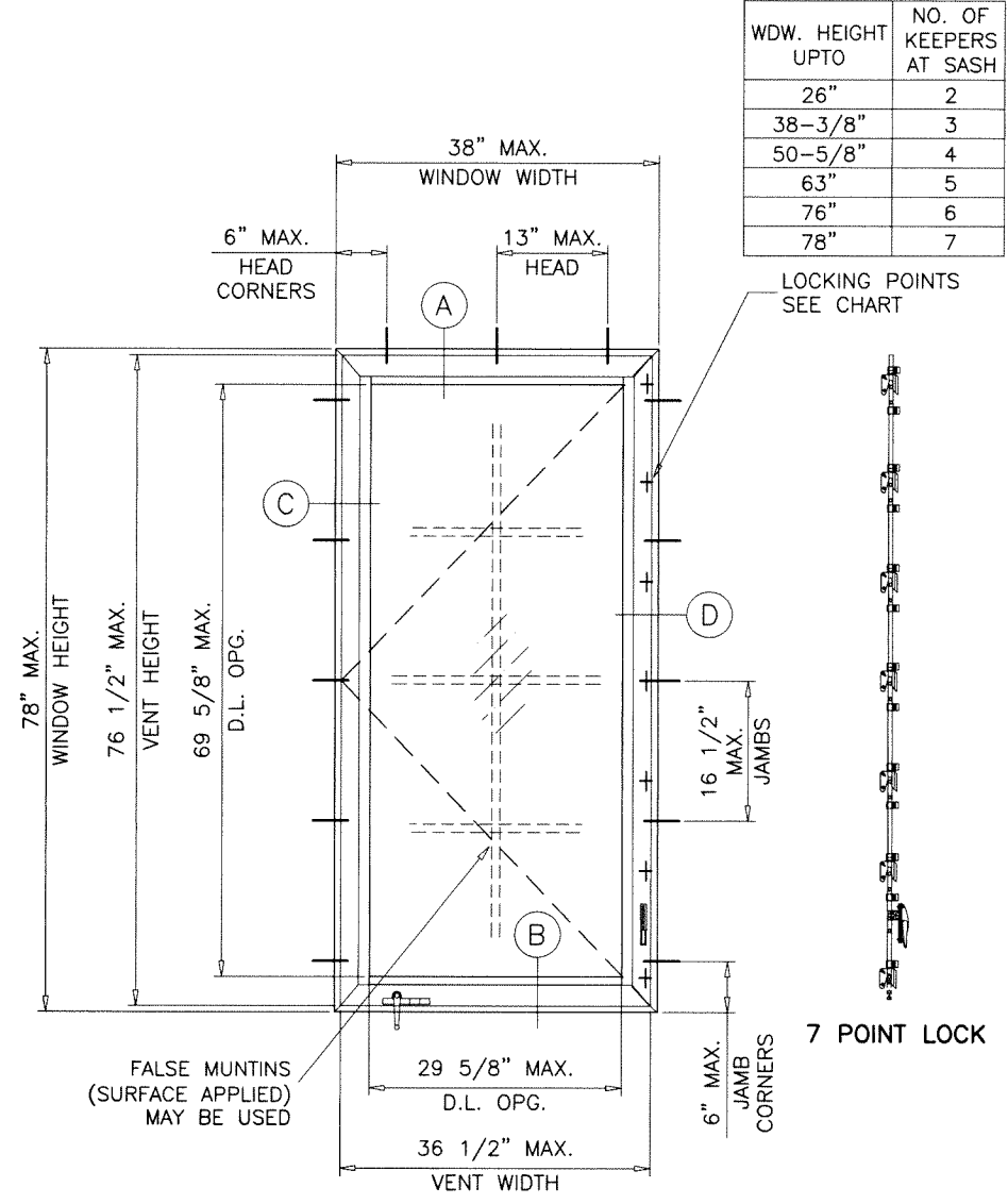
TYPICAL ELEVATION
