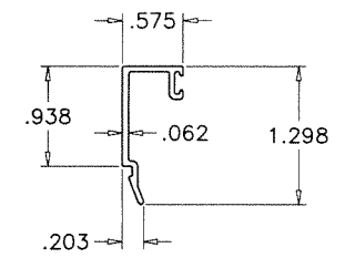
③ GLAZING BEAD (LAM. GLASS)
