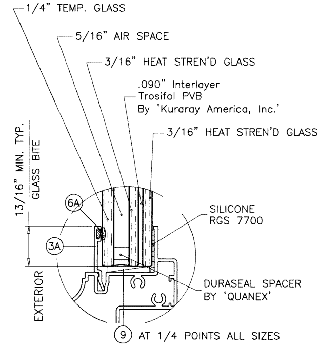
GLASS TYPE 'C' 1" OVERALL INSUL. LAM. GLASS
