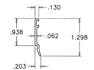
③A GLAZING BEAD (INSUL. LAM. GLASS)
