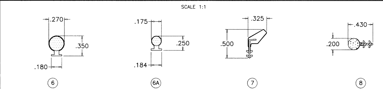
⑥ VENT EXTERIOR W'STRIPPING ⑥A GLAZING SPACER (LAM. GLASS) ⑦ GLAZING SPACER (INSUL. LAM. GLASS) ⑧ VENT INTERIOR W'STRIPPING ⑧ FRAME W'STRIPPING
