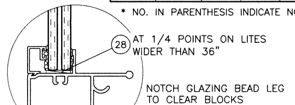
7/16" OVERALL LAM. GLASS TYPE 'F'
